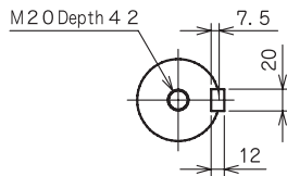
Keyed shaft
