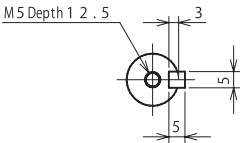
Keyed shaft
